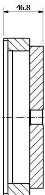
For front oil seal
